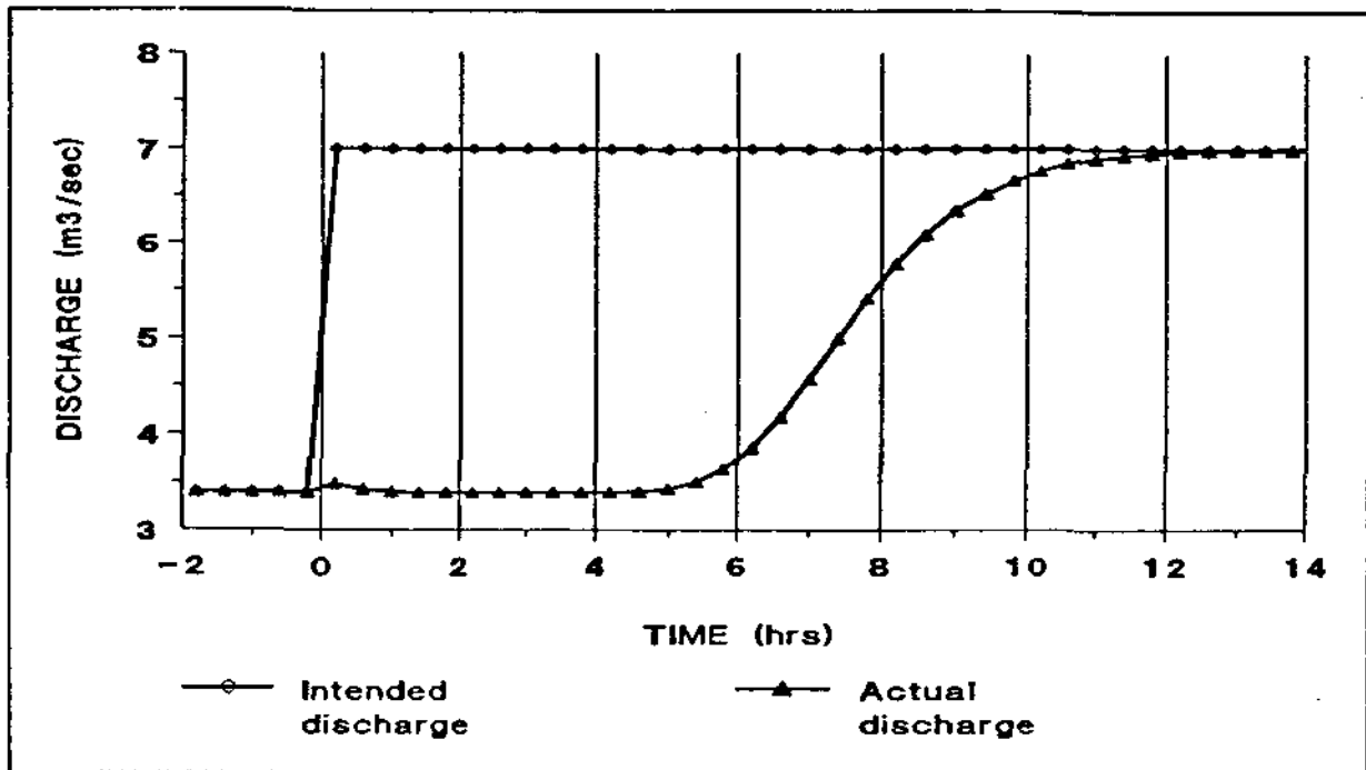
Figure 8: Response time of the system at bifurcation point (step 1)
