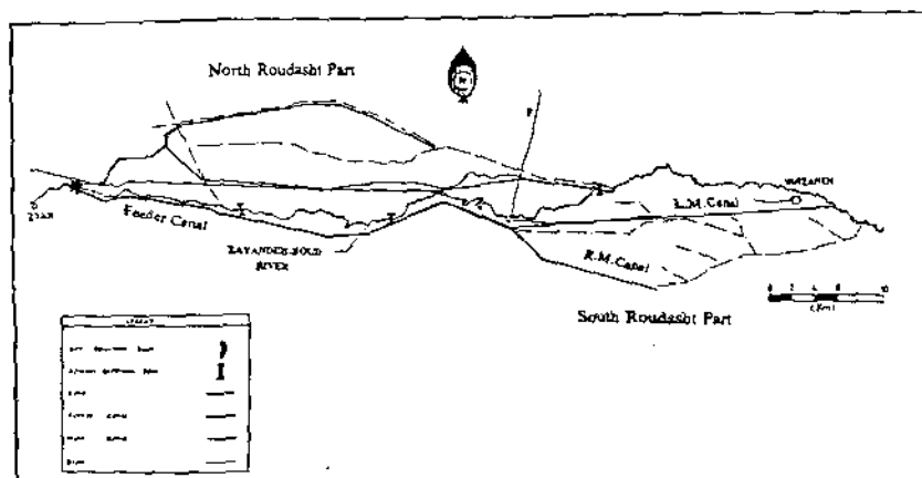
Figure 4: Roudasht Irrigation System
